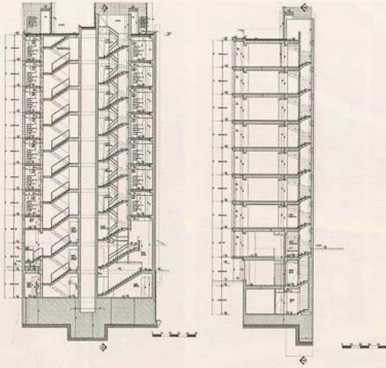
Kesitler Sections
